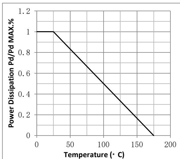
Fig.3 Power Dissipation
