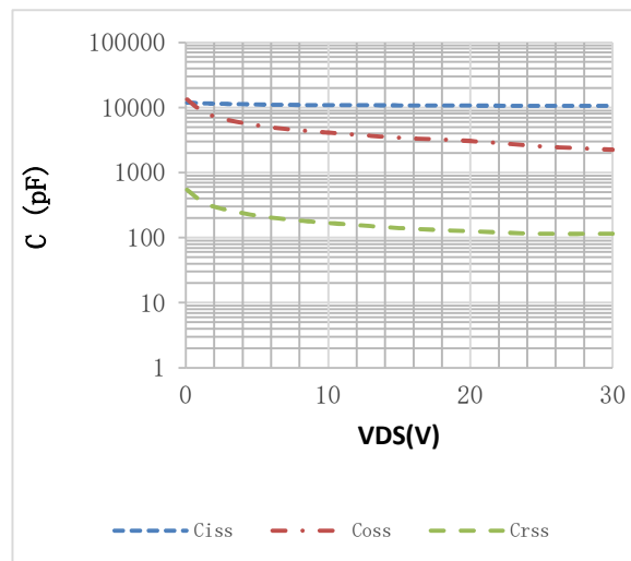
Fig.2 Capacitance Characteristics
